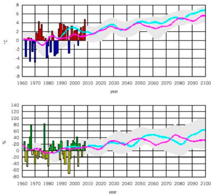
Figure 6.4 Presentation of data from observations of historical trend in the climate and how it may develop during the 21st century. Data present the deviation from the mean value for 1961-1990. Scenario results are stated as running averages. The grey area represents simulated variations. Stockholm County is shown as an example, with winter temperature in the top diagram and winter precipitation in the bottom diagram 50 .
