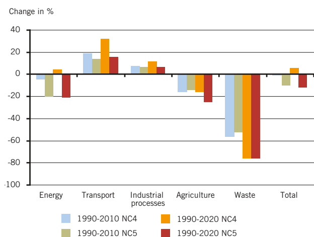
Figure 5.3 Percentage trend in emissions between 1990 and 2010 and 2020 according to the projections in NC4 and NC5, total and by sector.
