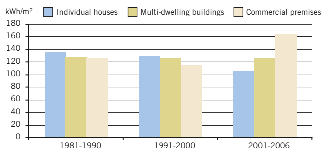
Figure 2.16 Energy use for heating in homes and commercial buildings constructed 1981-1990, 1991-2000, 2001-2006 17
